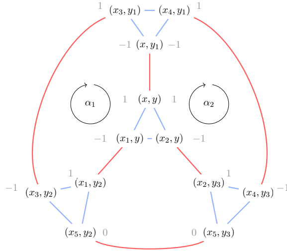
FIGURE 5.2. A 0-chain of \mathcal{O}_{12} characterizing decoupled fractions for the model \mathcal{G}_\lambda where the weights are written in grey next to their corresponding vertex.
