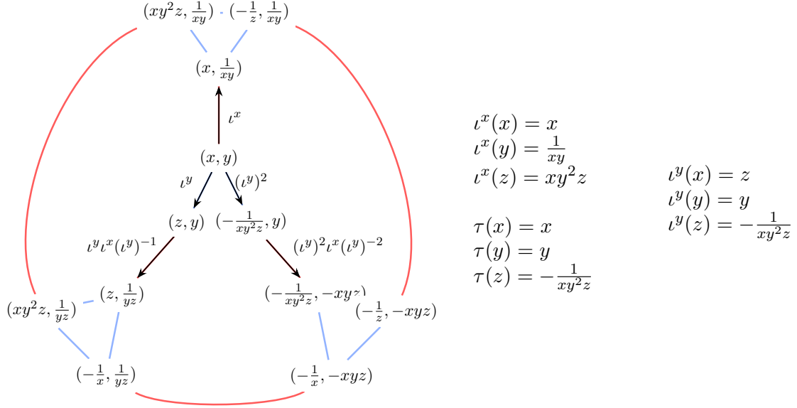
FIGURE 3.3. The elements of I_x and I_y for the model \mathcal{G}_\lambda
