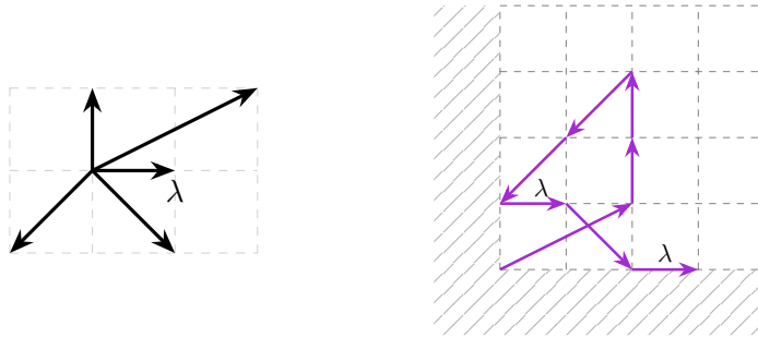
FIGURE 1.1. The weighted model \mathcal{G}_\lambda along with an example of a walk of size 8, total weight \lambda^2 and ending at (3,0)
